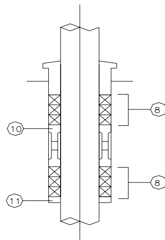
Fig. 5-7 SQUARE TYPE MOLD PACKING STRUCTURE
