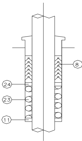
Fig. 5-6 TEFLON V-PACKING STRUCTURE
