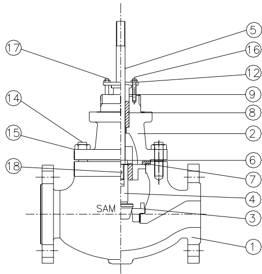
Fig. 5-11 Internal structure and parts name
